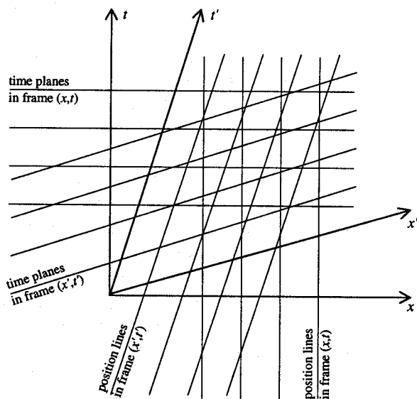
Figure 4. Position lines and time planes in two reference frames. Time in (x',t') “takes up” space in (x,t) and vice versa.
