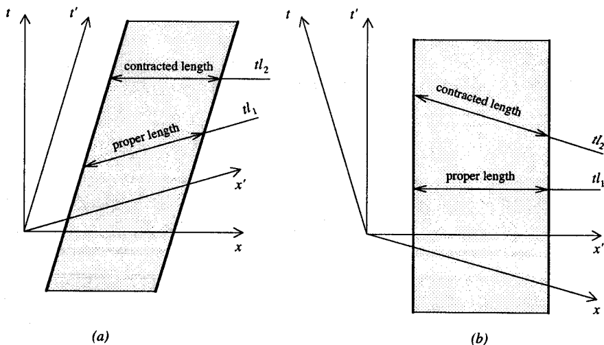
Figure 3. Lorentz contraction in special relativistic space-time. (a) and (b) represent the same state of affairs. For convenience, both pairs of coordinate axes, that is (x, t) and (x', t') , are included in both diagrams. The lengths of the pole in the two frames are not drawn to scale.
