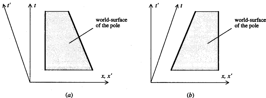
Figure 1. A contracting pole in two inertial reference frames. For convenience, both pairs of coordinate axes, (x, t) and (x', t') , are included in both diagrams.
