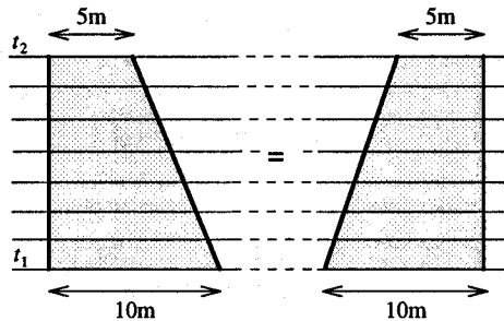
Figure 2. The contracting pole in Galilean space-time.
