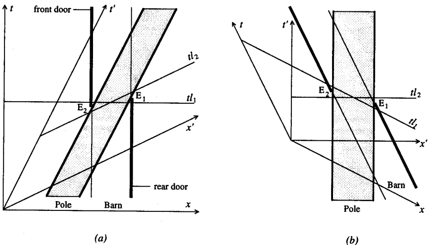
Figure 7. The pole is shorter than the barn in the barn rest frame (perspective tl_1 ) and longer than it in the pole rest frame (perspective tl_2 ). (a) and (b) represent the same state of affairs in relativistic space-time. The lengths of the pole and barn are not drawn to scale here.
