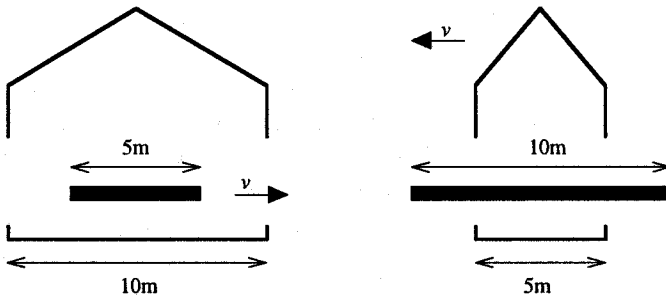
Figure 6. The Pole and Barn scenario: (a) in the barn's rest frame; (b) in the pole's rest frame.
